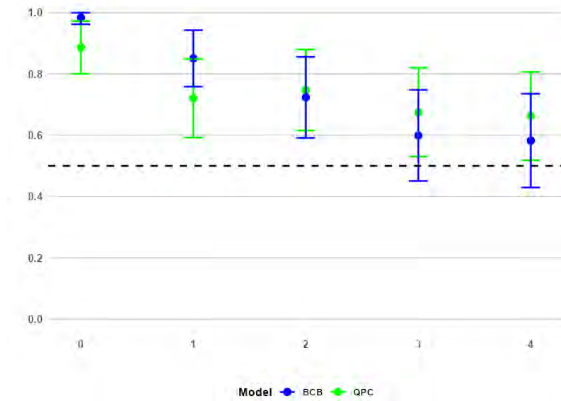
Figure 5.5: Displays the AUC values for QPC and BCB's conditional probability that inflation will be outside the bounds at a given horizon h . Plot includes 95% confidence intervals computed via DeLong method, and a dashed gray line at 0.5, representing the threshold for a random classifier. Probabilities are derived from predictive distributions from 2013:Q4 to 2024:Q4
