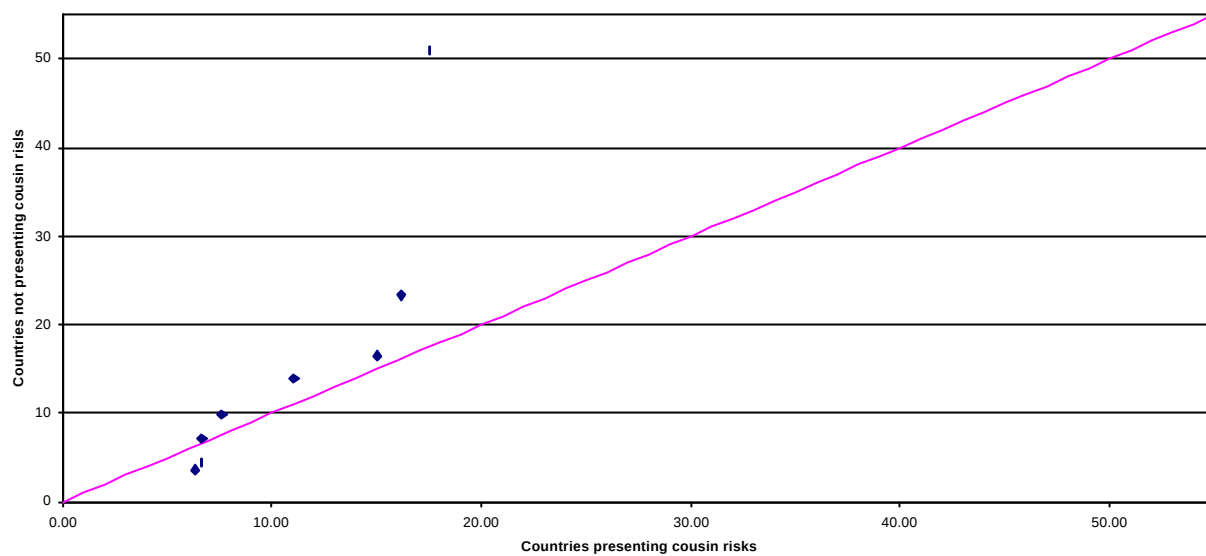
QQ-plot: International Reserves
