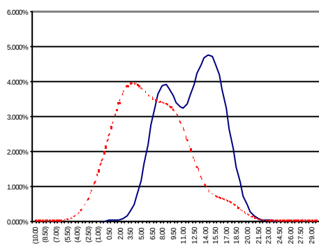
Non-Parametric Kernel Density: Mean Import Tariff Countries Presenting Cousin Risks vs Countries NOT Presenting Cousin Risks
