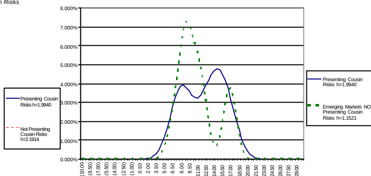
Non-Parametric Kernel Density: Mean Import Tariff Countries Presenting Cousin Risks vs Emerging Countries NOT Presenting Cousin Risks
