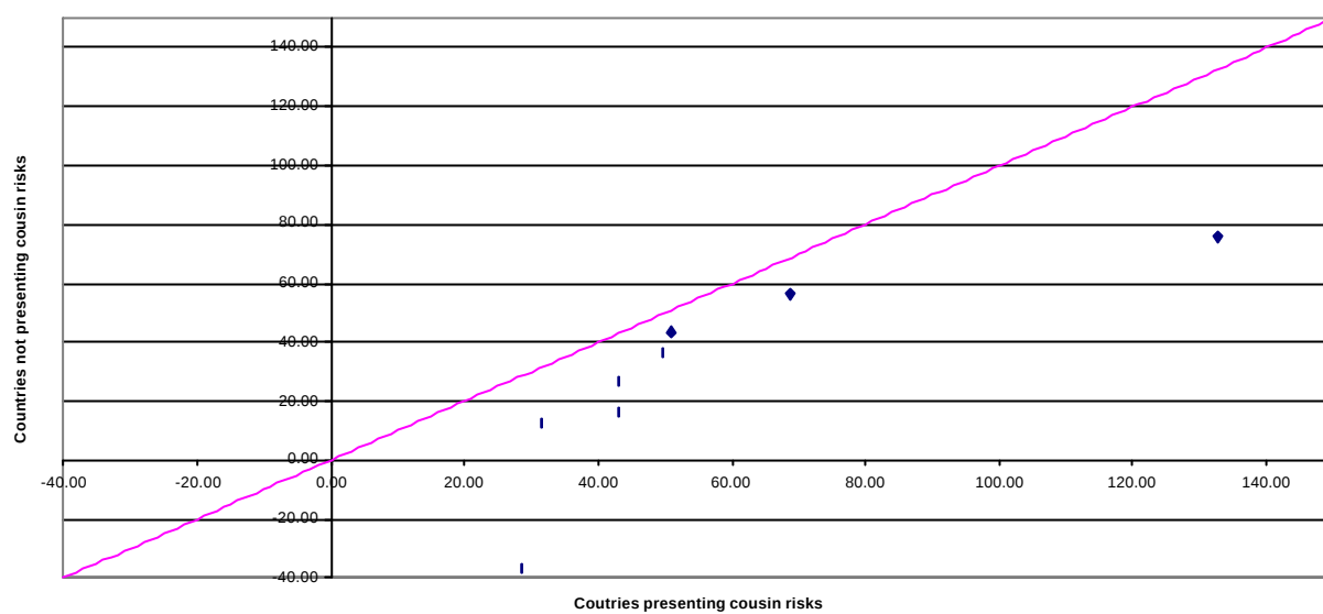
QQ-plot: Total Public Debt
