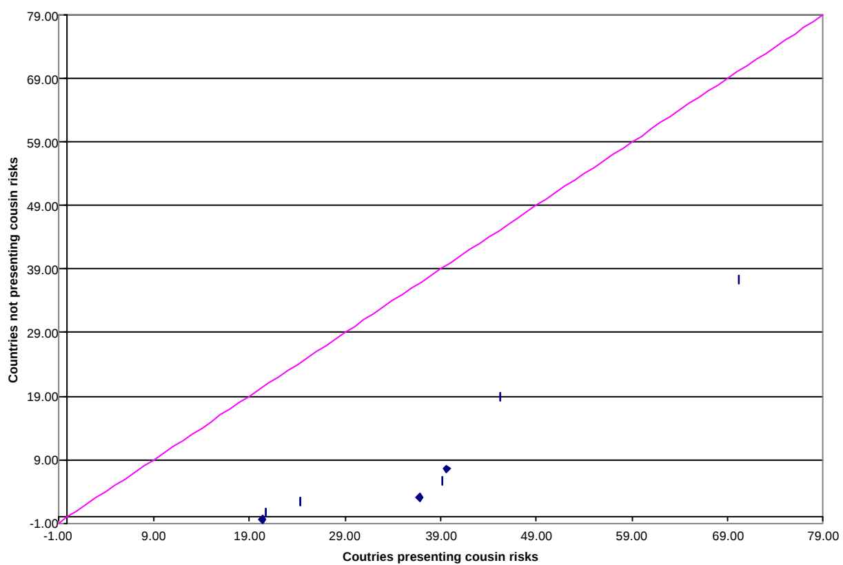
QQplot: External Government Debt
