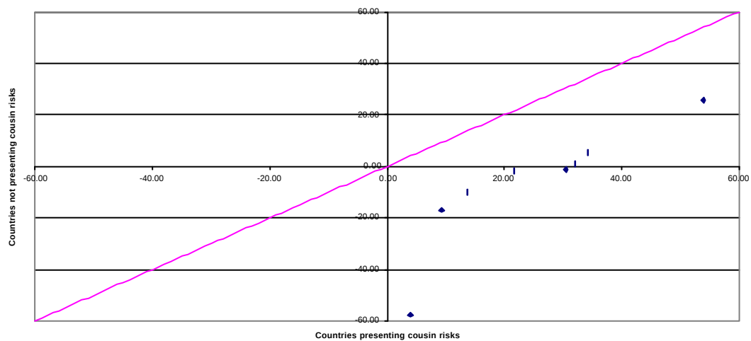
QQ-plot: Govt. External Debt - International Reserves
